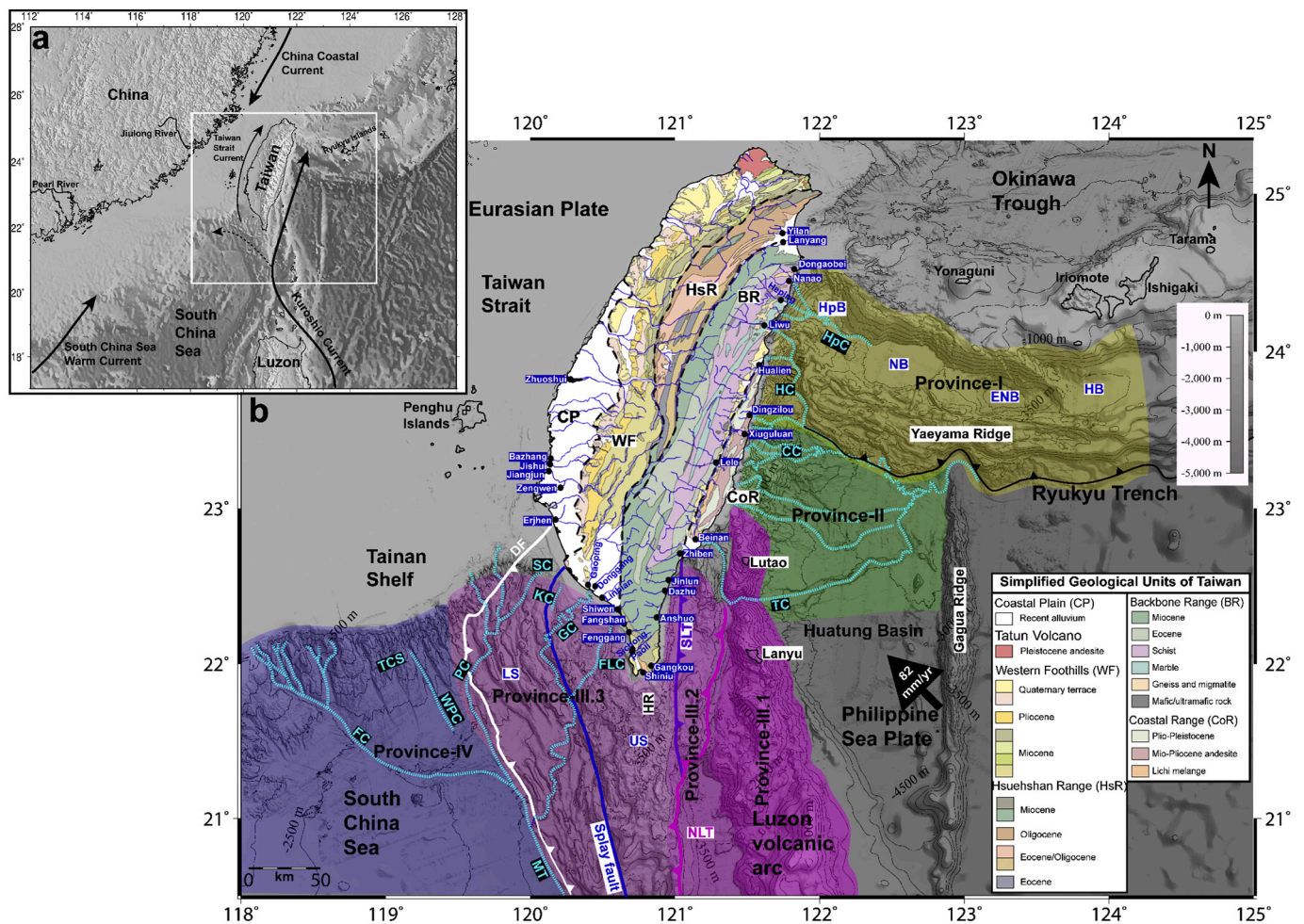
Fig. 1. (a) Map of Taiwan and its vicinity showing the oceanic current flow patterns. The location of the study area is marked by a white rectangle. (b) Geological map of Taiwan (after Chen, 2000) and shaded relief bathymetry offshore Taiwan. Major faults, canyons, and river sediment sampling locations (black circles) are shown on this map. The classified provinces are marked with different colours. Abbreviations: BR: Backbone Range, CC: Chimei Canyon, CoR: Coastal Range, CP: Coastal Plain, DF: Deformation Front, ENB: East Nanao Basin, FLC: Fangleiao Canyon, FC: Formosa Canyon, GC: Gaoping Canyon, HB: Hateruma Basin, HC: Hualien Canyon, HP: Hengchun Peninsula, HR: Hengchun Ridge, HpB: Hoping Basin, HpC: Hoping Canyon, HsR: Hsuehsan Range, KC: Kaohsiung Canyon, LC: Manila Trench, NB: Nanao Basin, NLT: North Luzon Trough, PC: Penghu Canyon, SC: Shousan Canyon, SLT: Southern Longitudinal Trough, TC: Taitung Canyon, TCS: Tainan Continental Slope, WF: Western Foothills, WPC: West Penghu Canyon and the splay fault bordering the lower-slope (LS) and upper-slope (US) domains.
