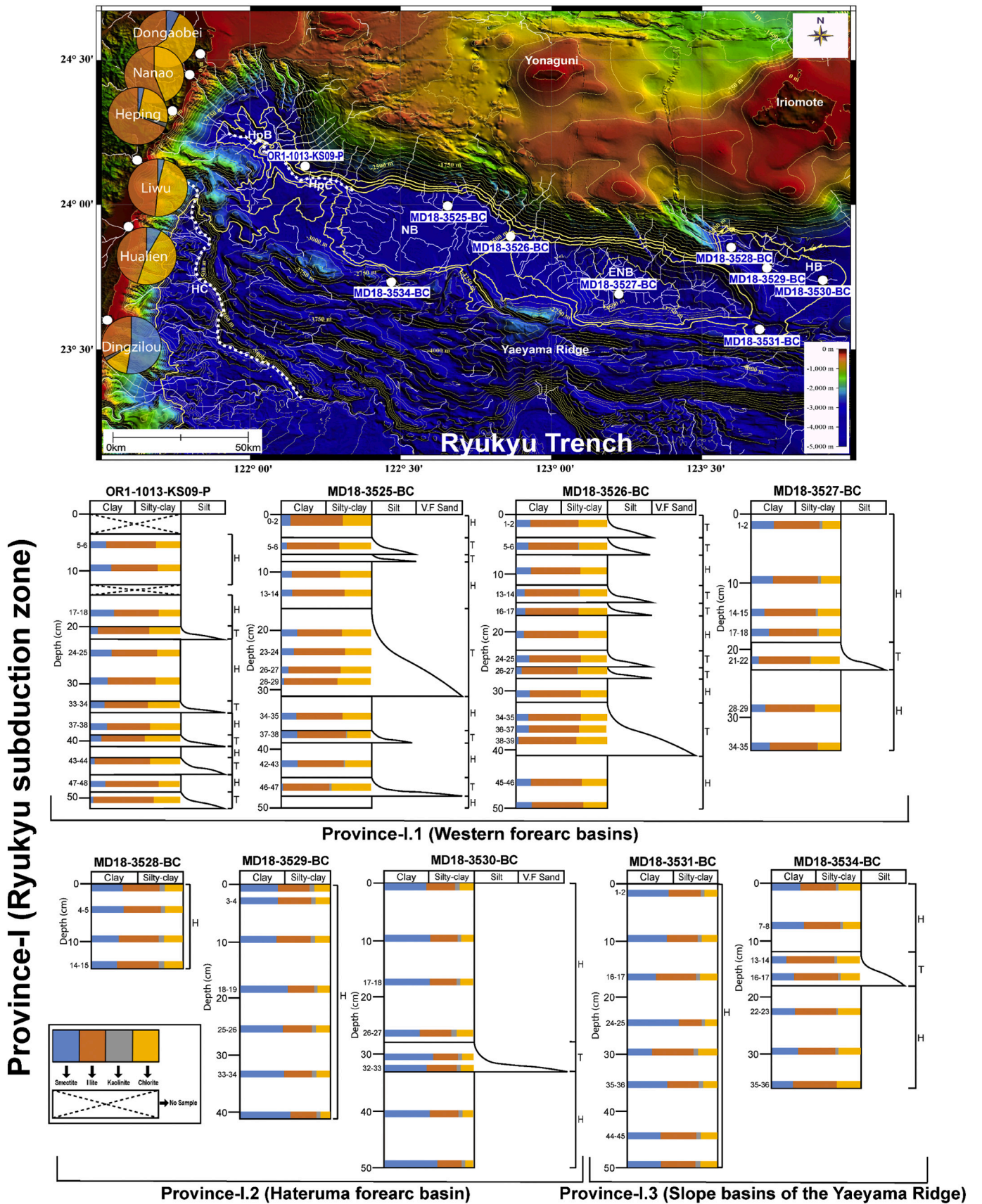
Fig. 6. Figure showing drainage patterns with distributions of clay mineral percentages in surrounding Taiwanese river sediments and lithological descriptions with vertical clay mineral distributions of the studied cores in Province-I. Abbreviations: ENB: East Nanao Basin, HB: Hateruma Basin, HC: Hualien Canyon, HpB: Hopping Basin, Hpc: Hopping Canyon, NB: Nanao Basin. Contour lines show the elevation in 250-m intervals.
