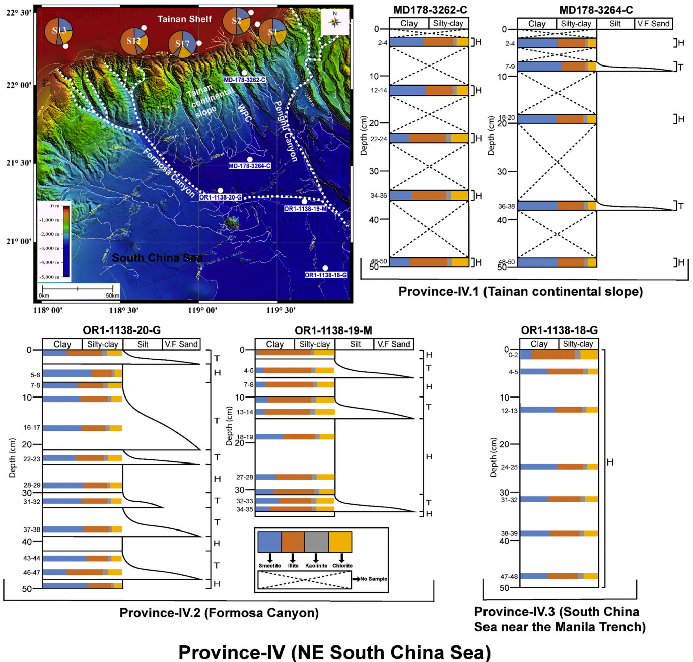
Fig. 11. Figure showing drainage patterns with distributions of clay mineral percentages in surrounding Taiwanese river sediments and lithological descriptions with vertical clay mineral distributions of the studied cores in Province-IV. Abbreviation: WPC: West Penghu Canyon. Contour lines show the elevation in 250-m intervals.
