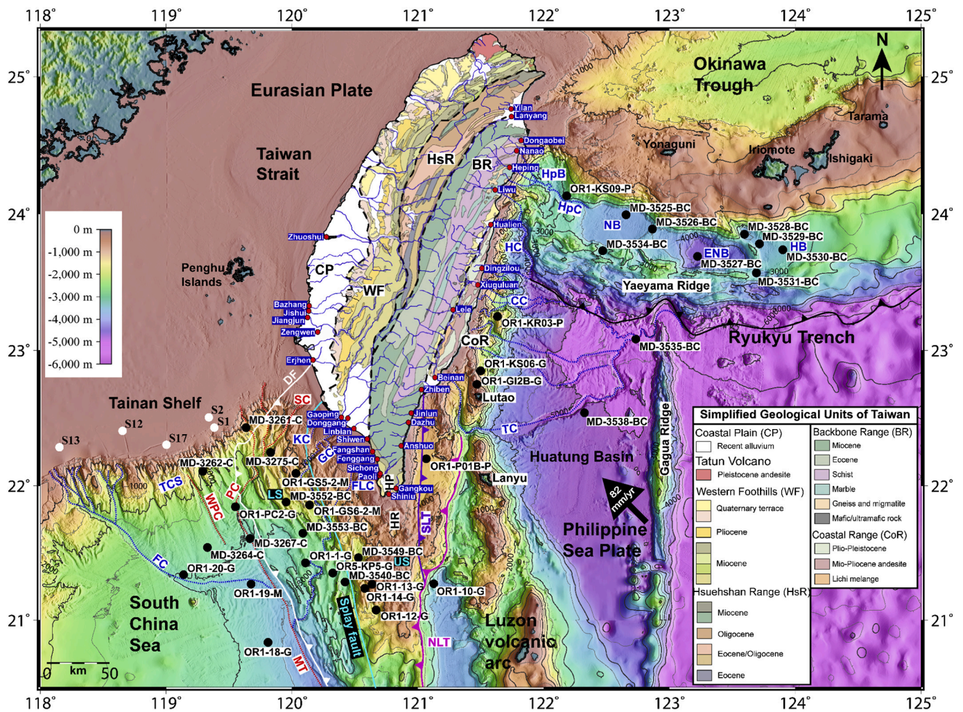
Fig. 2. Shaded relief bathymetric map around offshore Taiwan, showing Major faults, canyons, location of sediment cores (black circles), and location of sediment grabs from the southern Taiwan Strait (white circles). Geological map of Taiwan showing river sediment sampling locations (red circles). See Fig. 1 for abbreviations. (For interpretation of the references to colour in this figure legend, the reader is referred to the web version of this article.)
