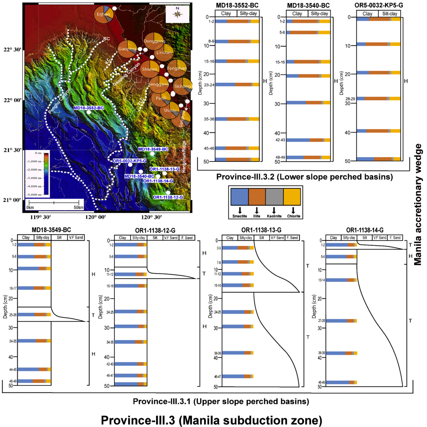
Fig. 9. Figure showing drainage patterns with distributions of clay mineral percentages in surrounding Taiwanese river sediments in Province III.3 and lithological descriptions with vertical clay mineral distributions of the studied cores in Provinces: III.3.1 and III.3.2. Abbreviations: FLC: Fangliao Canyon, KC: Kaohsiung Canyon, SC: Shougan Canyon. Contour lines show the elevation in 250- m intervals.
