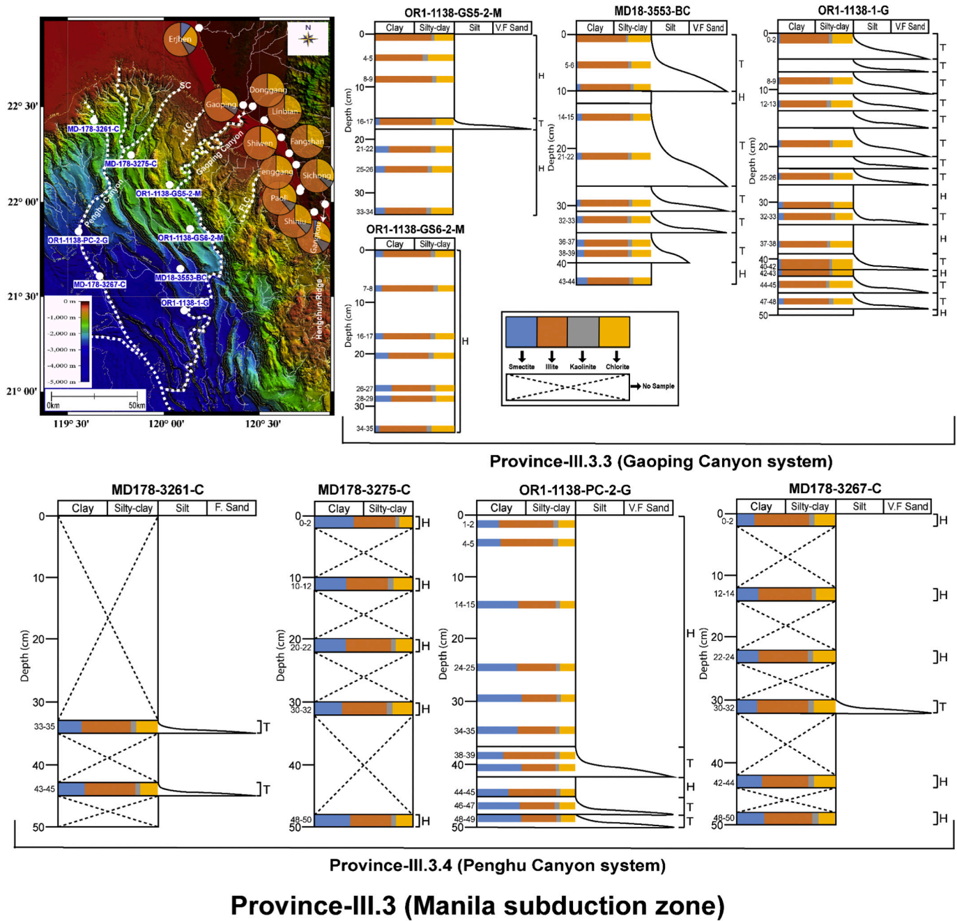
Fig. 10. Figure showing drainage patterns with distributions of clay mineral percentages in surrounding Taiwanese river sediments in Province III.3 and lithological descriptions with vertical clay mineral distributions of the studied cores in Provinces: III.3.3, III.3.4. Abbreviations: FLC: Fangliao Canyon, KC: Kaohsiung Canyon, SC: Shousan Canyon. Contour lines show the elevation in 250- m intervals.
