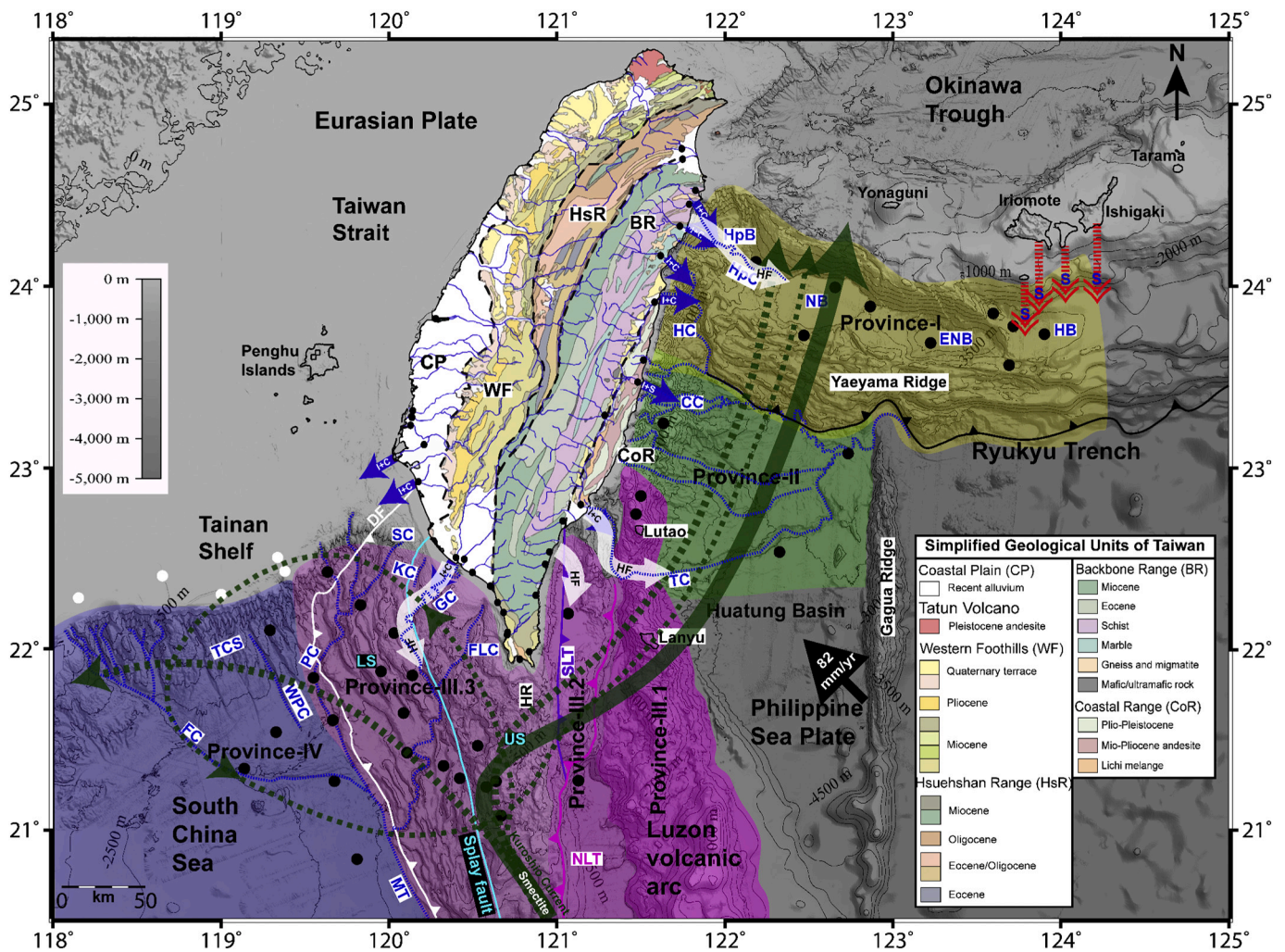
Fig. 14. Map showing a synopsis of spatial sediment transport processes/paths in the deep seas around Taiwan based on characteristic clay minerals from various source terrains. The arrows in black (solid and dashed) showing the different types of Kuroshio intrusion (modified from Caruso et al., 2006). Abbreviations: HF: Hyperpycnal flows, I: Illite, C: Chlorite, S: Smectite. See Fig. 1 for other abbreviations.
